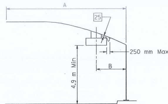
SIGN PLACEMENT
