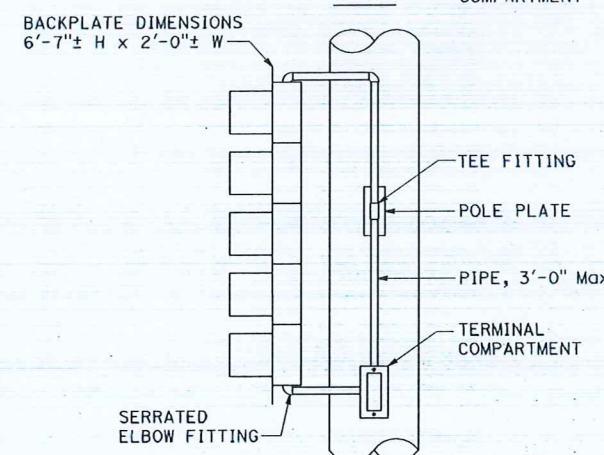
SV-1-T WITH 5 SIGNAL SECTIONS
