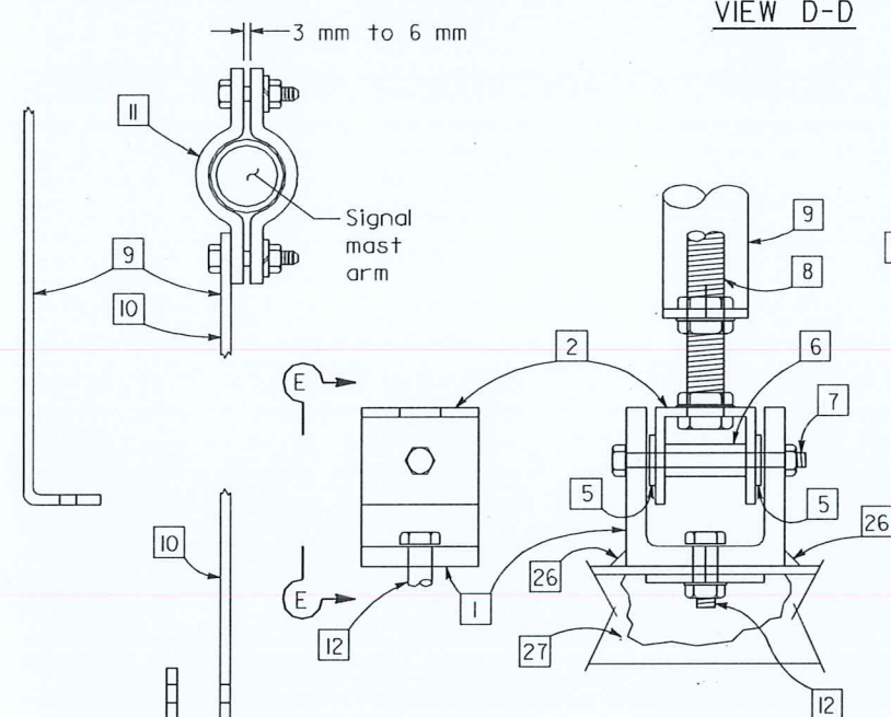
VIEW E-E
