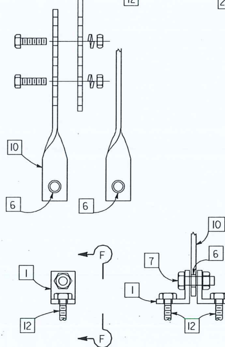
VIEW F-F
