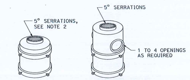
TOP MOUNTINGS For 4 NPS pipe, see Note 2.
