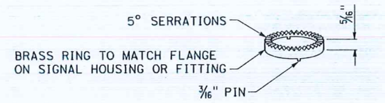
LOCK RING Use where locking ring is not integral with signal housing or fitting.
